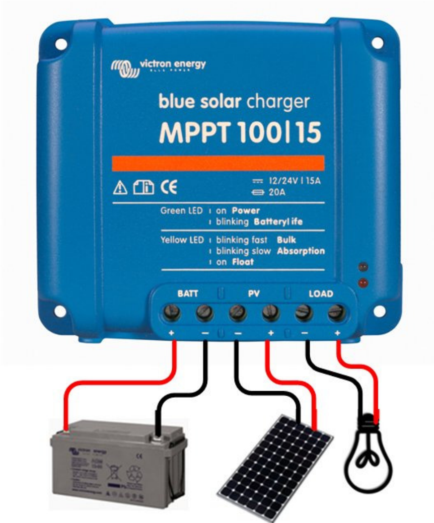
Figure 3: Power connections
